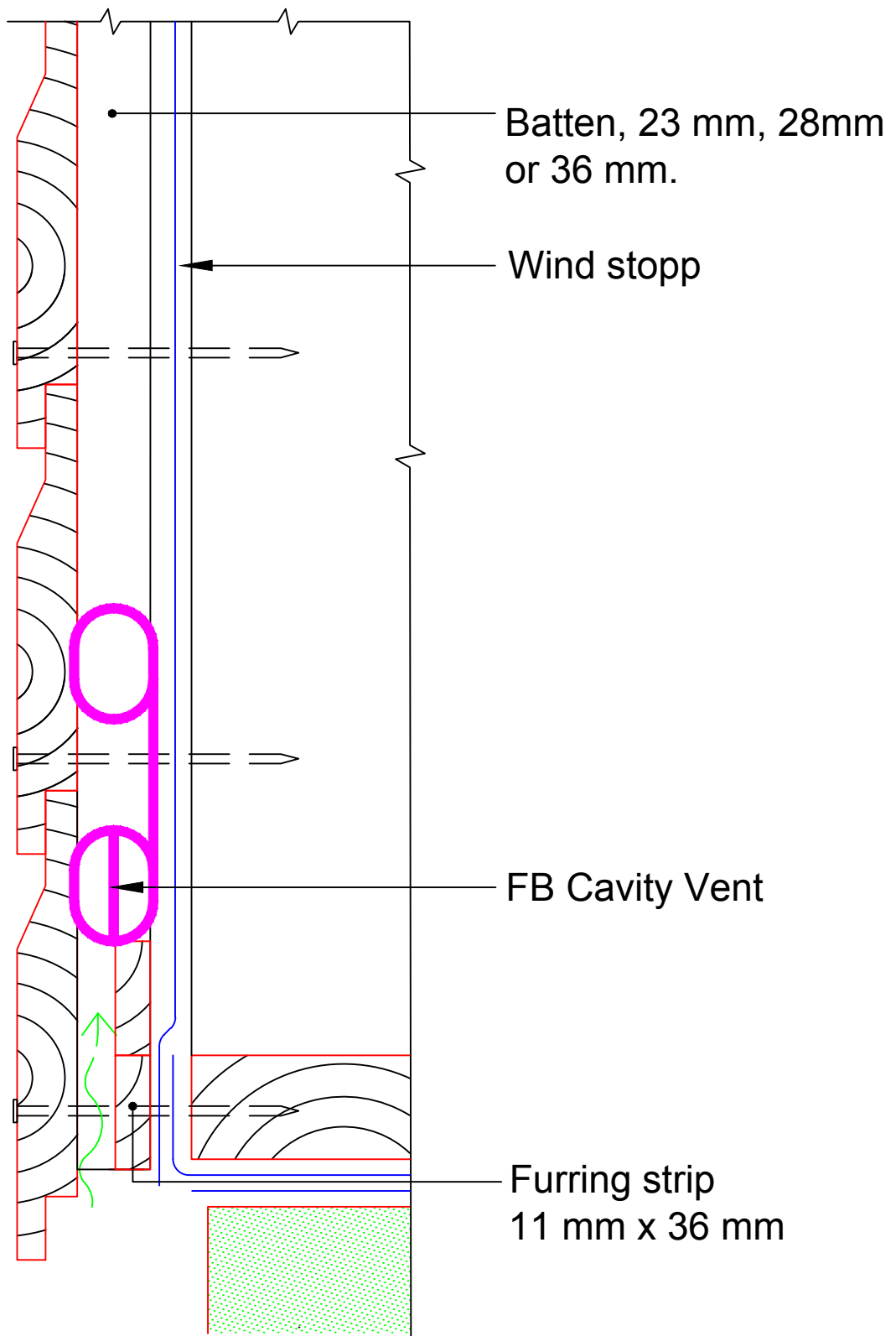
Horizontal cladding
